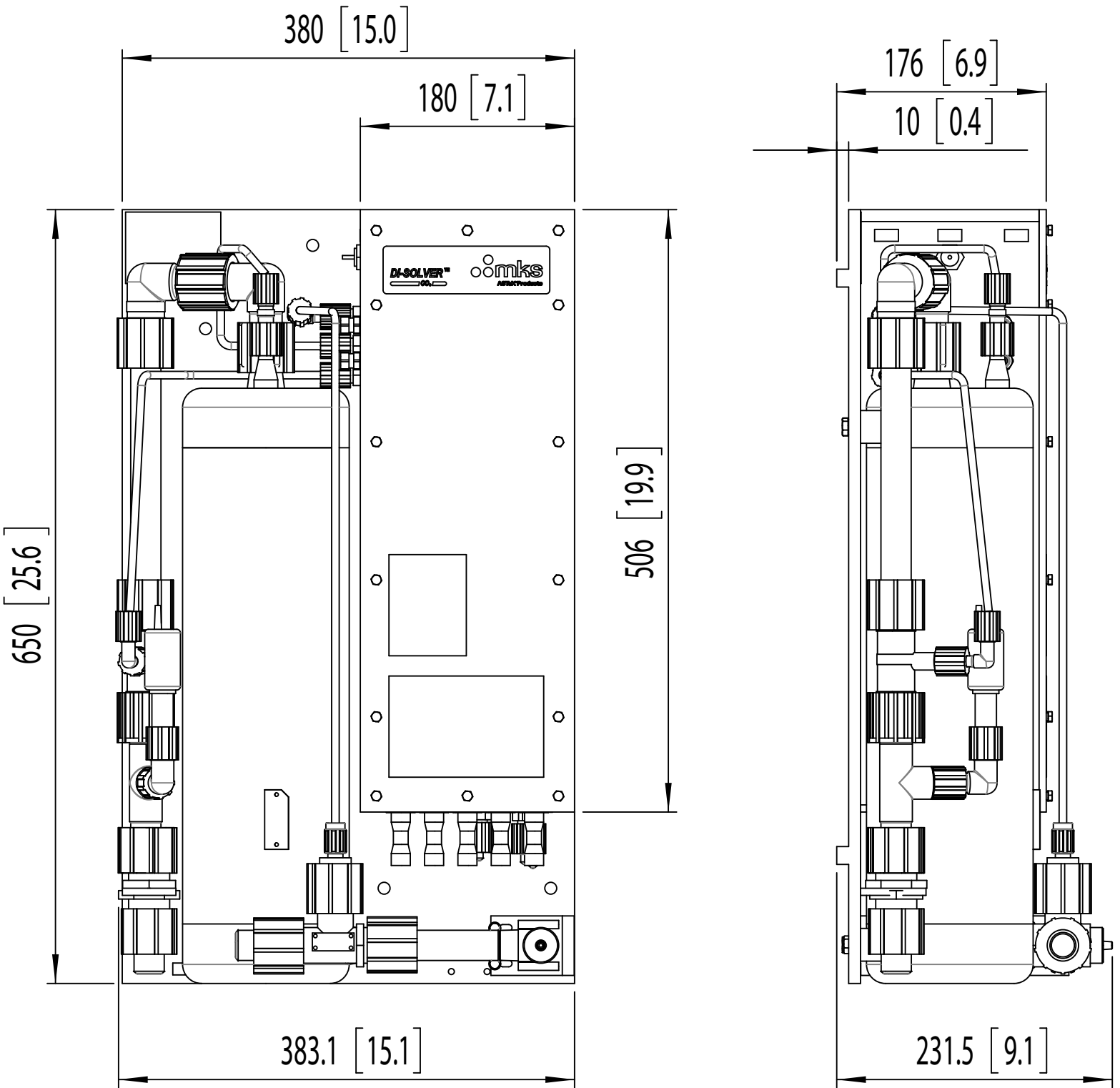
Dimensional Drawing with Flaretek® Fittings Unless otherwise specified, dimensions are nominal values in millimeters (inches referenced).
